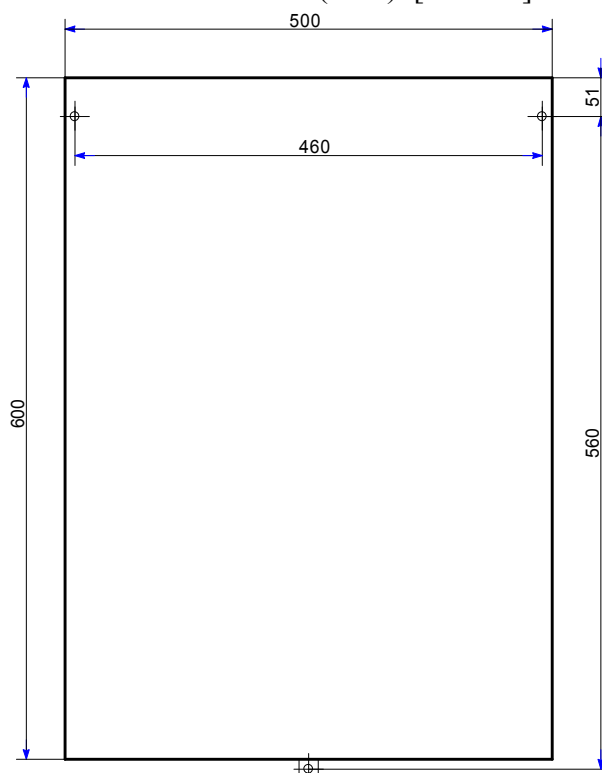
СВТ64.142.000-09(..-13) [32 - 80А]*
