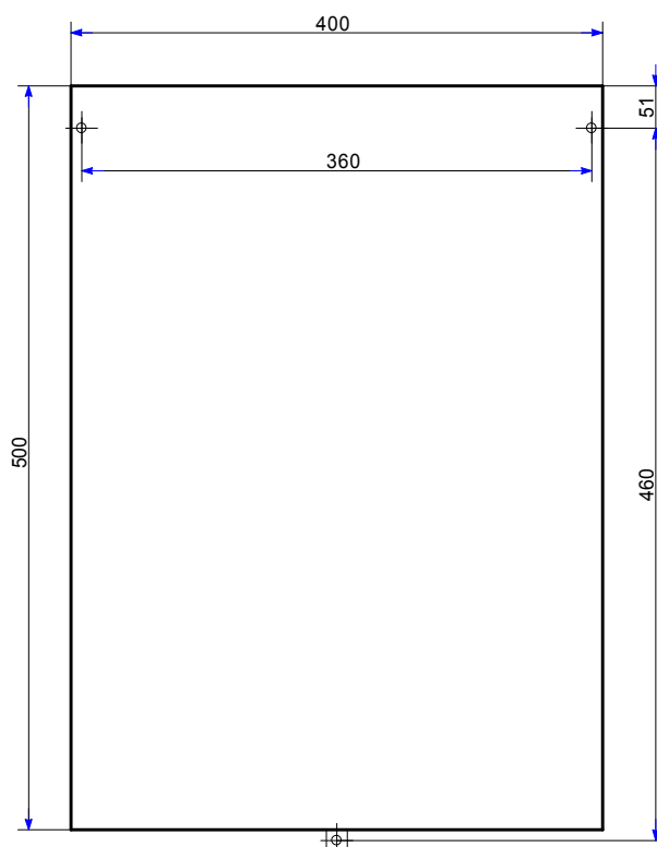
СВТ64.142.000-01(..-08) [1 - 25А]*
